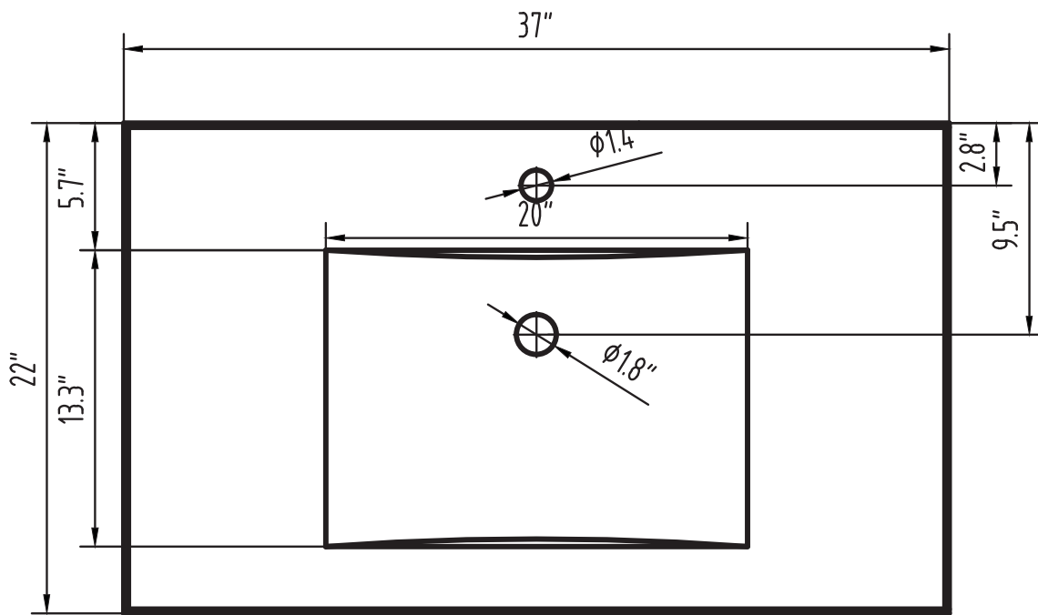
TOP VIEW
